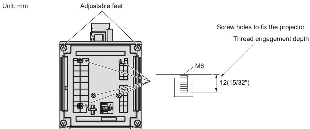
Adjustable feet Adjustable feet Positions of screw holes to fix projector and adjustable feet
